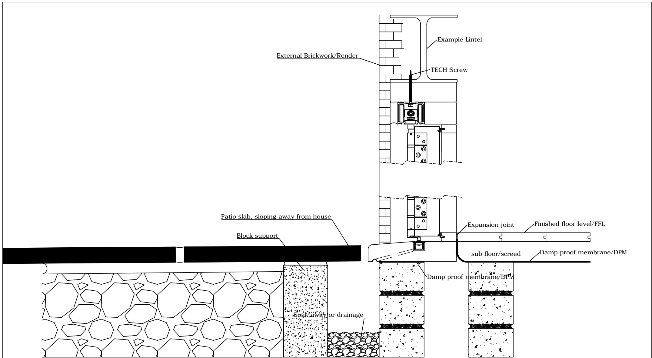
Valdi Ltd - Top Hung Folding Sliding Doors - Standard Timber Drip Sill - Outward opening - Raised Patio Construction
